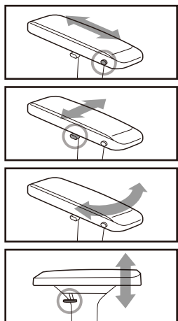
Adjustable armrest
